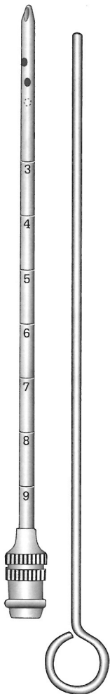
Frazier MWH-25-470 3 mm \varnothing Silver plated MWH-25-475 2 mm \varnothing Gold plated 12 cm / 4 3/4"
